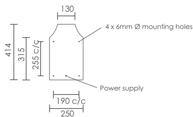
Mounting Plate Detail
