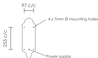
Mounting Plate Detail
