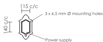
Mounting Plate Detail
