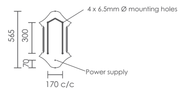
Mounting Plate Detail
