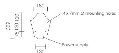
Mounting Plate Detail
