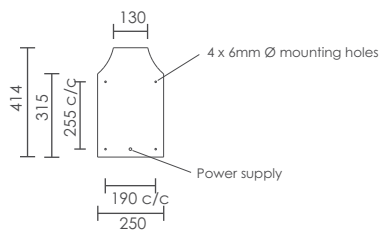
Mounting Plate Detail
